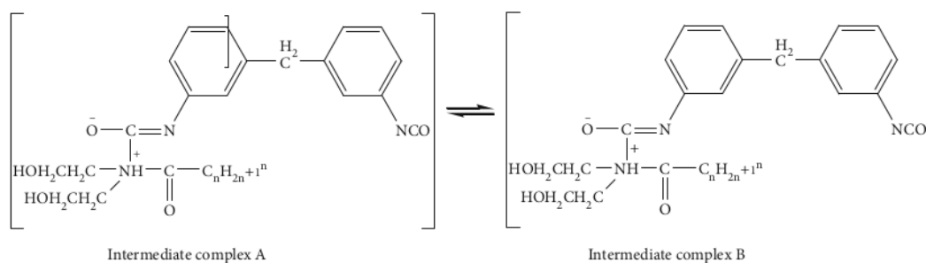
FIGURE 4: The formation of intermediate complexes.
