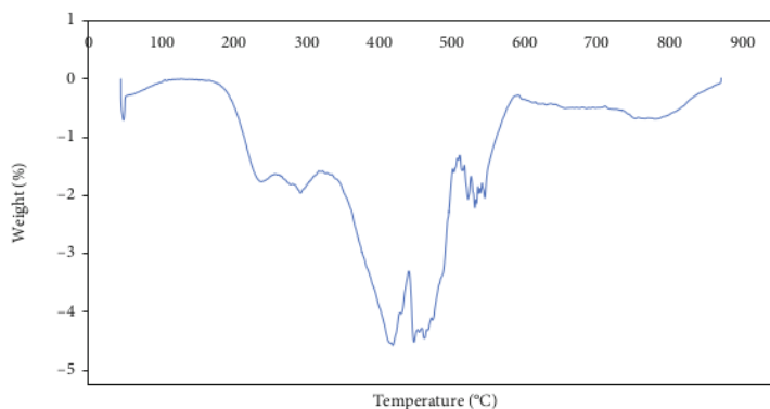
FIGURE 7: DTG thermogram of polyurethane film.
