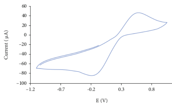
FIGURE 9: The voltammogram of SPE-PU modified electrode after analyzed using cyclic voltammetry technique.
