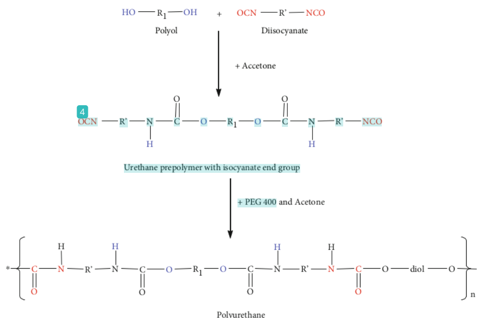
FIGURE 2: PU production via the prepolymerization method [41].
