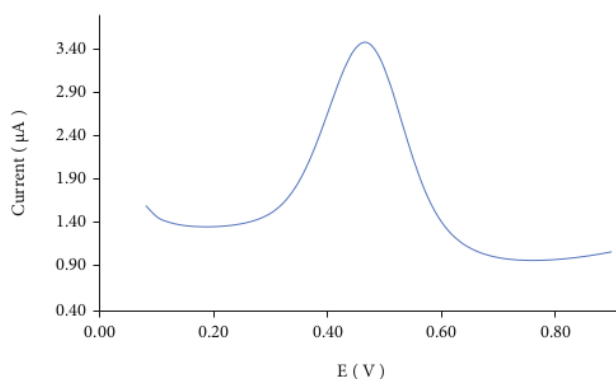
FIGURE 10: The voltammogram of SPE-PU modified electrode after analyzed using differential pulse voltammetry technique.
