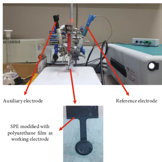
FIGURE 1: Potentiostat instrument to study the conductivity of SPE modified with polyurethane film using voltammetric approach: CV and DPV.
