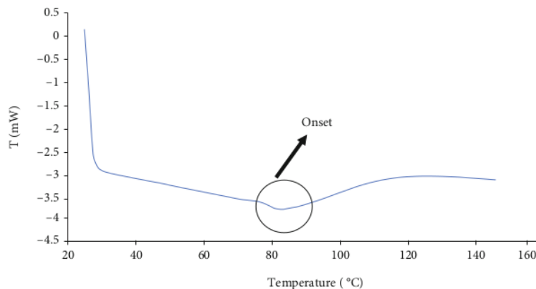
FIGURE 8: DSC thermogram of polyurethane film.
