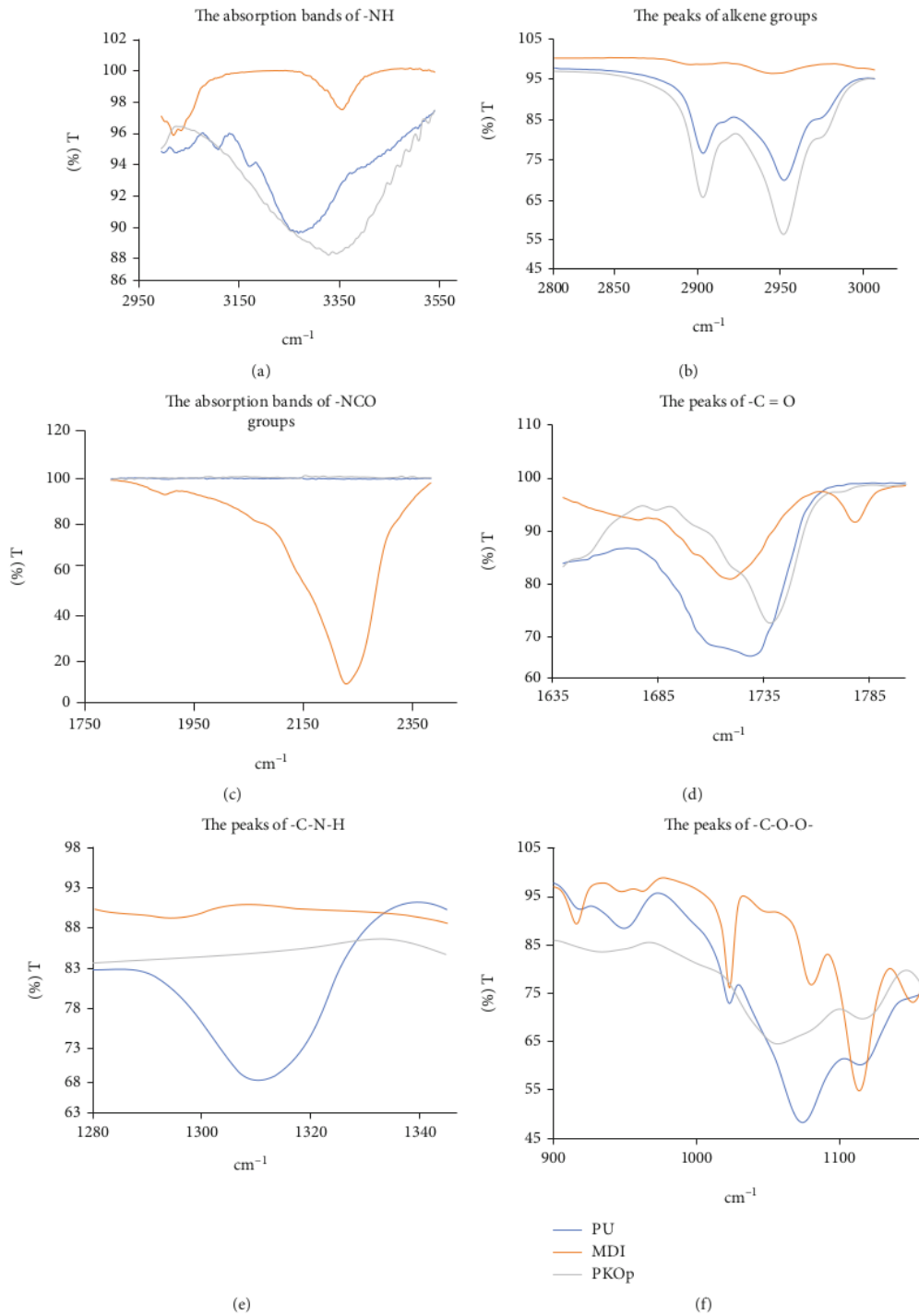
FIGURE 3: FTIR spectra of several important peaks between polyurethane, PKO-p, and MDI.
