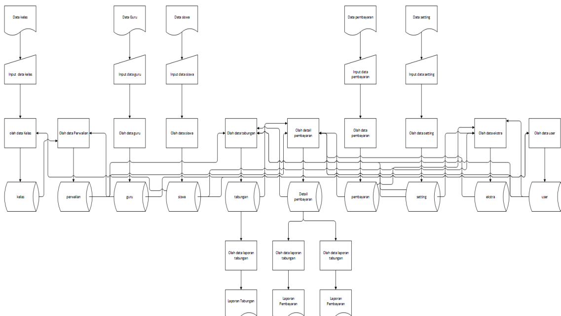
Gambar 2. Flowchart
